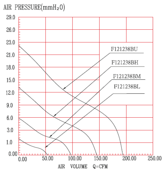
AIR FLOW-AIR PRESSURE(PERFORMANCE CURVES)
