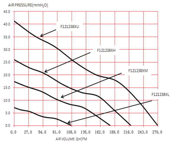
AIR FLOW-AIR PRESSURE(PERFORMANCE CURVES)
