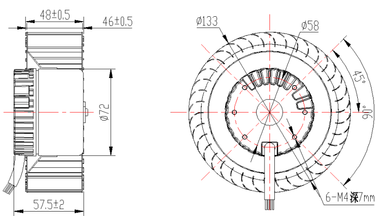
产品尺寸图 Product dimension drawing
