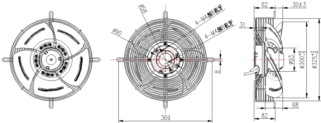
产品尺寸图 Product dimension drawing
