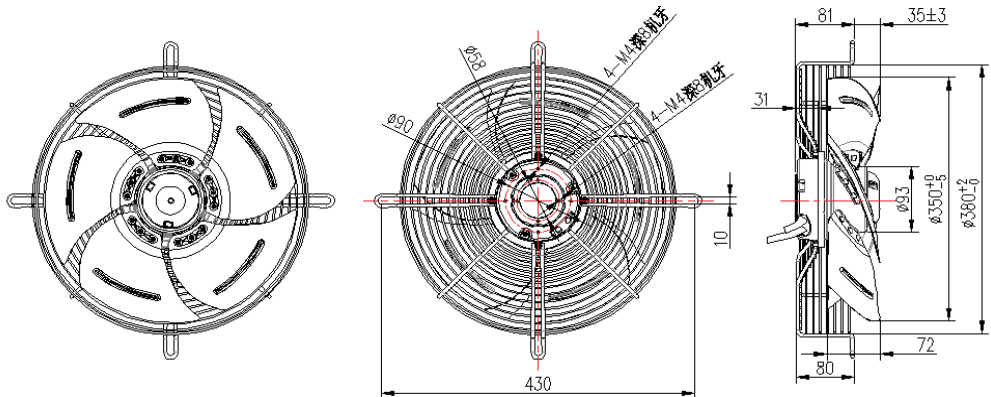
产品尺寸图 Product dimension drawing
